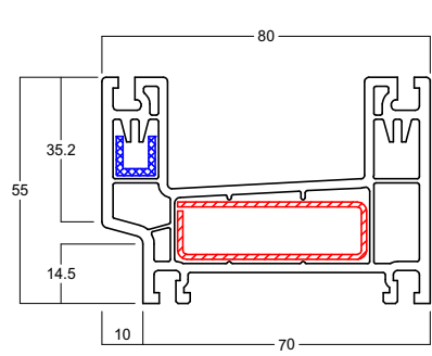
55mm Stepped Outer Frame Art No: 6054 Reinf V108 or V109
