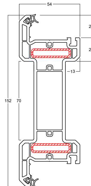
152mm Midrail Art No: 6049.D Black gasket Art No: 6049.L Silver gasket Reinf V081
