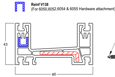
43mm Triple Track Outer Frame Art No: 6050 Reinf V155
