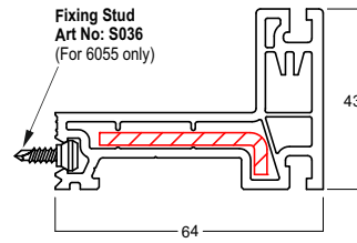
Triple Track Frame Adaptor Art No: 6055 Reinf V155
