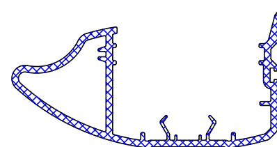
Alu Interlock/Pull Grip Art No: 9C58-1 White Art No: 9C58-1 Bronze (For Sash 6041 only)
