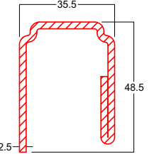
Reinf V355 (For 6041, enhanced) lx = 7.44
