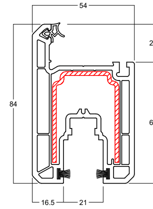
84mm Sash Art No: 6041.D Black gasket Art No: 6041.L Silver gasket Reinf V106
