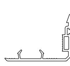
Sash Interlock Cover Art No: 6060 White Art No: 6060 Foiled Art No: 6060 Foiled on White (For PremiLine PRO only)
