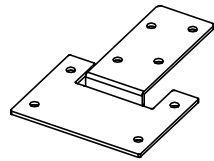
Frame Mech Joint Bracket Art No: 9C52 (For Frame 6052 only)
