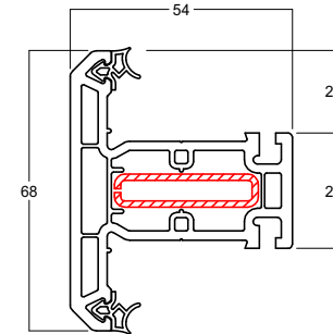
68mm Transom Art No: 6048.D Black gasket Art No: 6048.L Silver gasket Reinf V081
